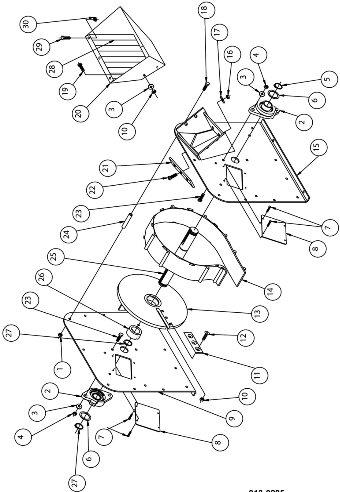
913-0285 CHIPPER BASIC MACHINE
