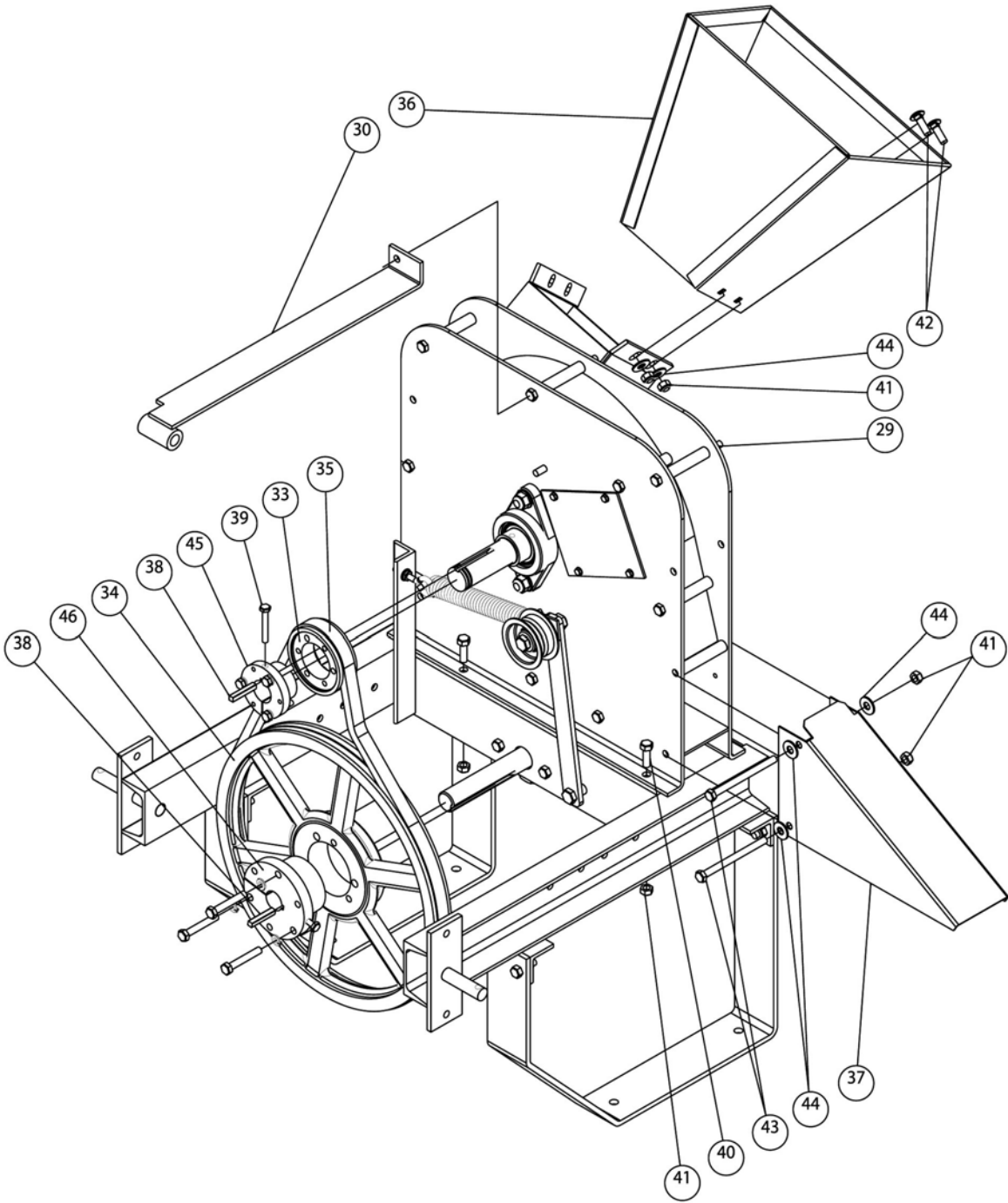
TPH-CHP BASIC & PULLEY ASSEMBLY
