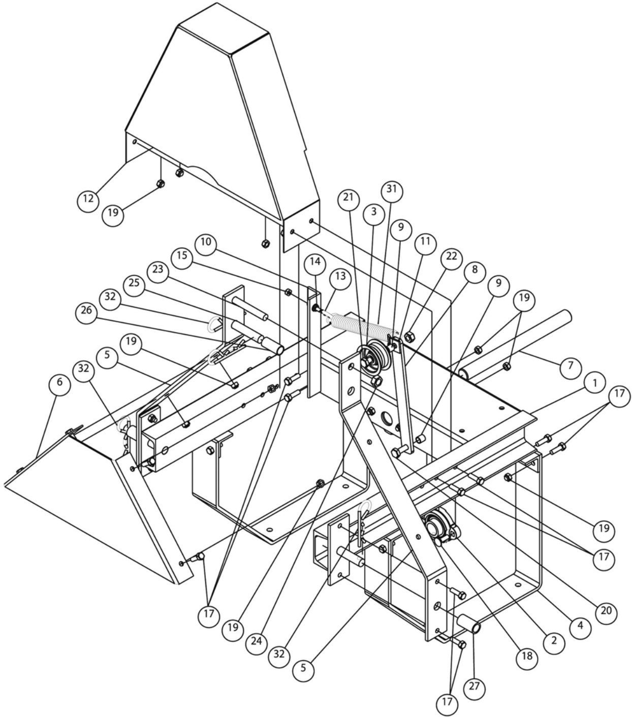
TPH-CHP FRAME ASSEMBLY
