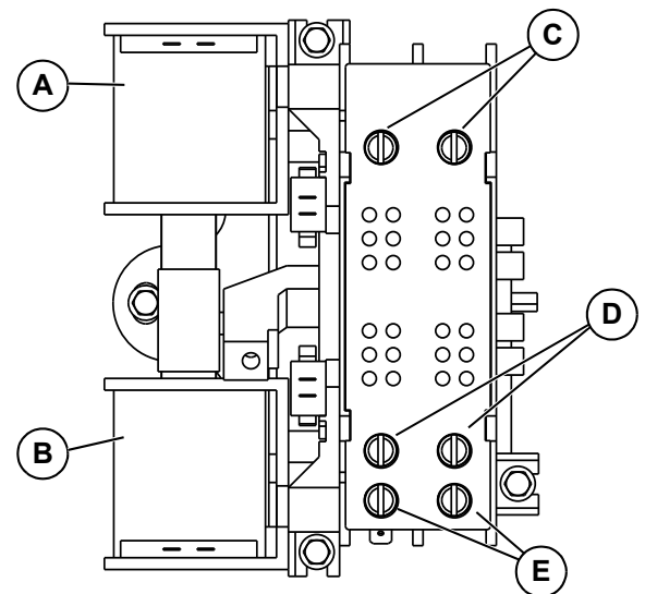
Figure 2-1. Typical Single-Phase ATS Transfer Mechanism
