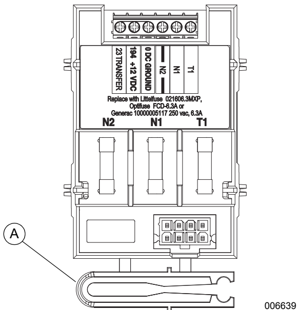
Figure 4-2. Fuse Removal and Installation Tool
