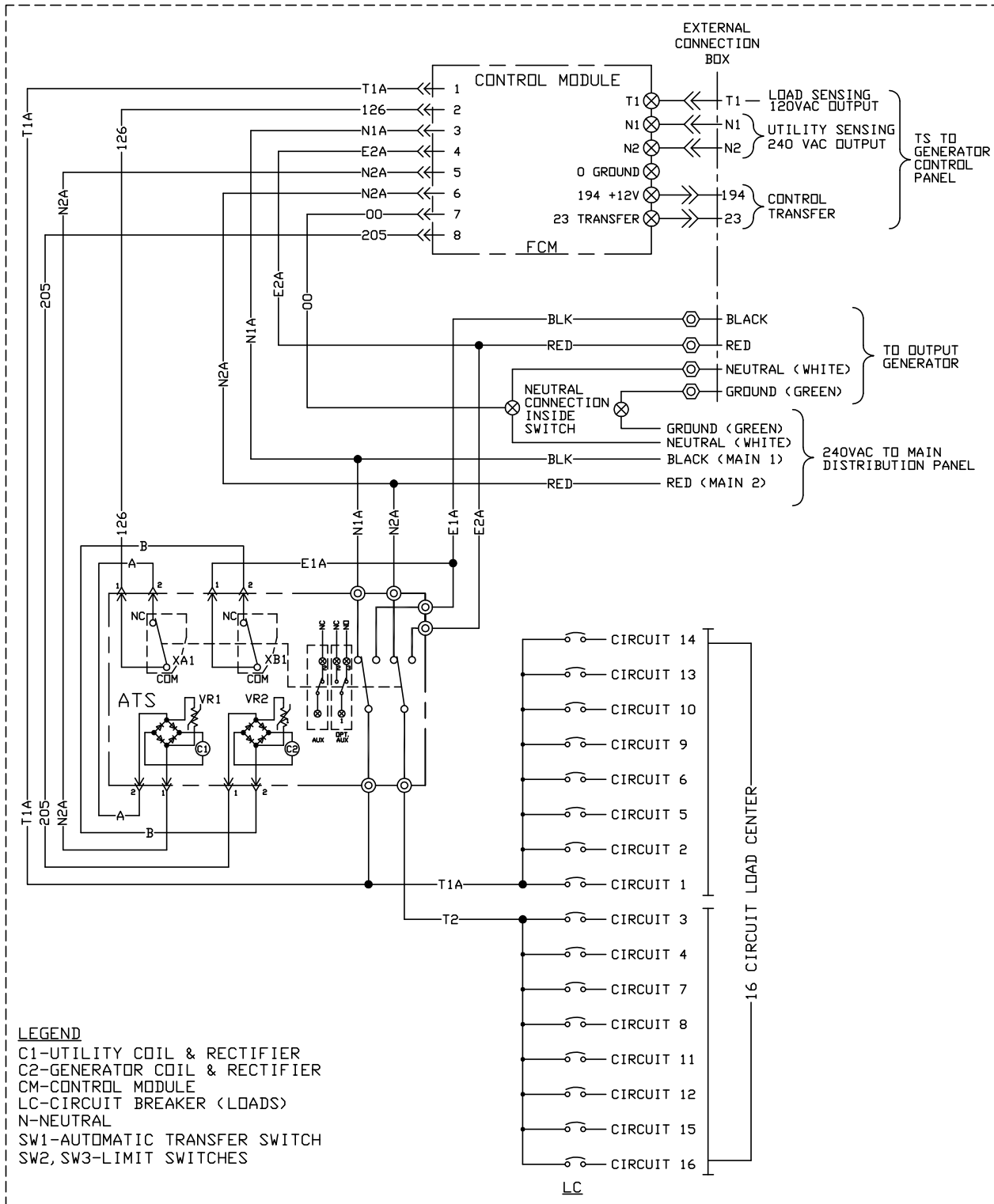
SCHEMATIC - DIAGRAM HSB TRANSFER SWITCH 100A DRAWING #:10000011443
