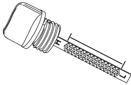
Figure 4-6. Oil Level
