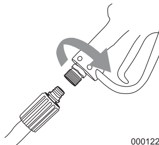
Figure 2-12. Connect High-Pressure Hose to Spray Gun
